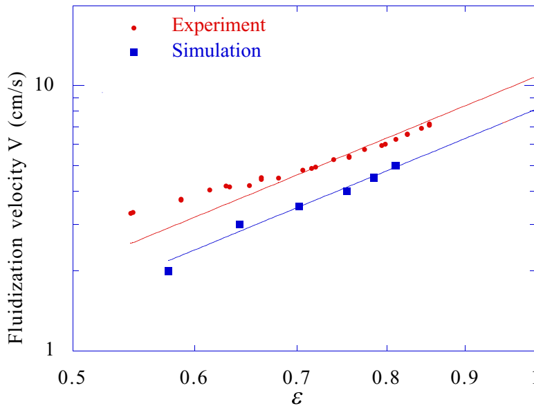
Figure 2(b). Data from Figure 2(a) plotted in a log-log plot. The slopes of the straight line are given by the Richardson-Zaki n = 2.39 . The blow-out velocities V_s(0) and V_e(0) are defined as the intercepts at \epsilon = 1 .
