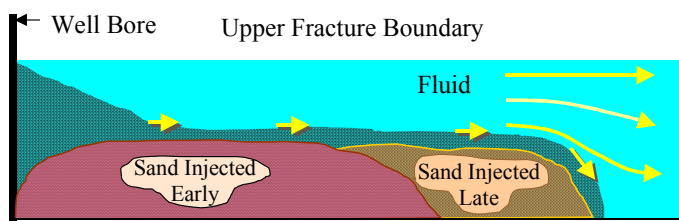
Figure 13. (Kern, Perkins and Wyant 1959) Sand transport in a fractured reservoir is different than the eroded bed of 300 particles in Figure 9(a) and 10(a) because particles are injected. The creation of algorithms to simulate continuous injection is one of our simulation projects.
