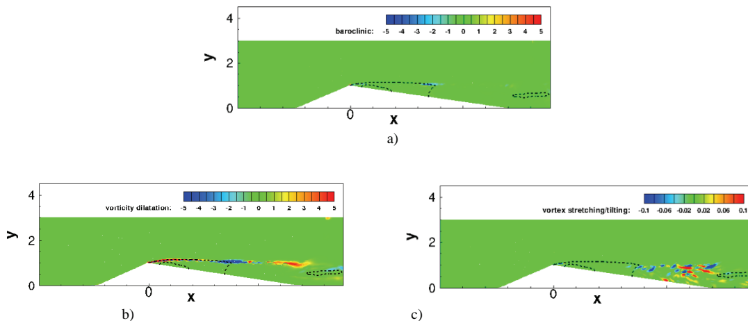
Figure 7. Vorticity budget: a) baroclinic production, b) vorticity dilatation and c) vortex stretching/tilting averaged along the span
