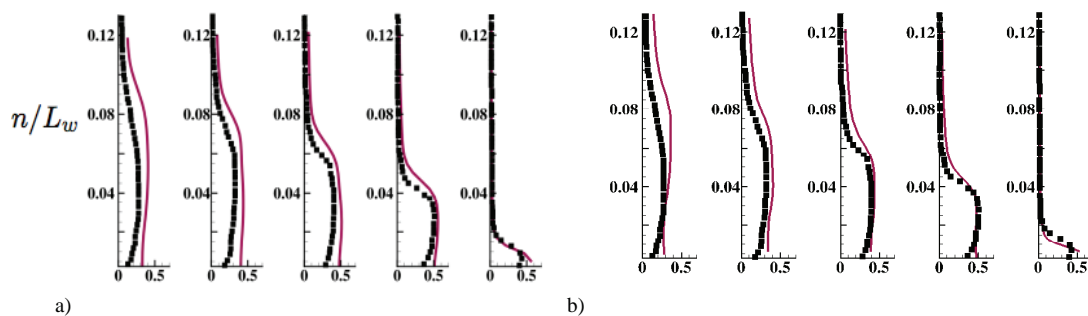
Figure 5. Surface normal profiles of the temporal average of spanwise averaged (for 3D) volume fraction data ( \langle \alpha \rangle_z ) at different stations along the wedge surface, s/L_w = 0.49, 0.37, 0.26, 0.14, 0.02 respectively from left to right Ganesh et al symbols [1], (-) LES.
