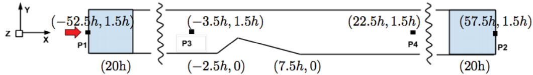
Figure 1. Schematic of the x - y plane of the computational setup (figure not to scale)
