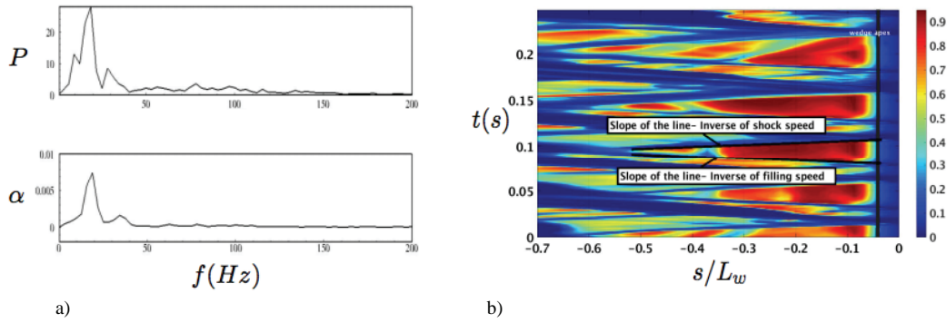
Figure 6. a) PSD of pressure and volume fraction taken inside cavity at 1.5h downstream of wedge apex. b) Contours of vapor volume fraction taken parallel to the surface of wedge for 0.25s (roughly 4-5 shedding cycles)
