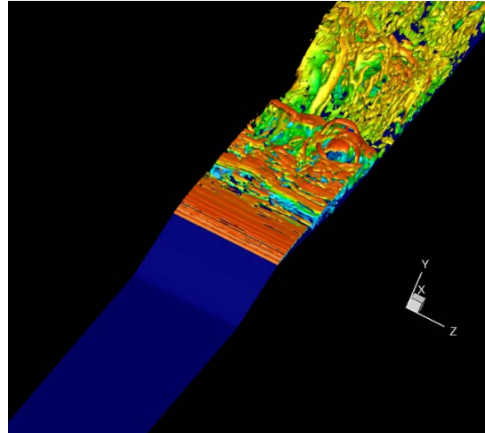
Figure 8. Iso-contours of Q Criterion colored by stream-wise velocity representing vortical structures.
