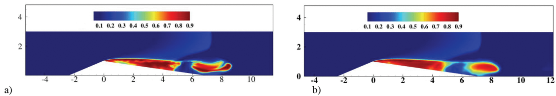
Figure 4. Instantaneous volume fraction contours in the a) symmetry plan ( z=0 ) and b) span-wise averaged.
