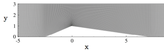
Figure 2. 2D-slice of the computational mesh close to the wedge (dimensions are in inches)
