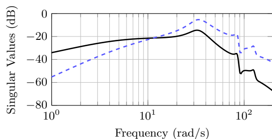
(b) Normalized singular values for deflection ( K S_1/\delta_{\max} —) and rate ( s K S_1/\delta_{\max} - - -).
