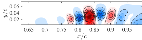
(b) Real part of C_{p'} TDMD mode at St = 2.06 .
