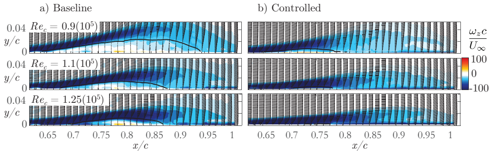
Figure 35: Time-averaged z -vorticity for separated flow subjected to adaptive LQR control computed from 4800 PIV snapshots. The mean recirculation region is denoted by a solid black line corresponding to \bar{u} = 0 . This shows that applying the adaptive feedback control using LQR gains significantly reduces the size of the separation region.
