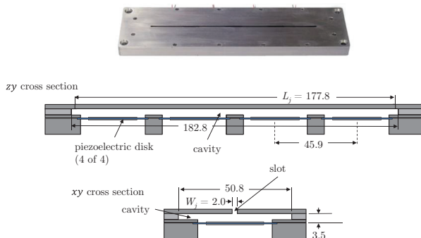
Figure 2: Photograph and schematic illustration of the ZNMF actuator (adapted from Griffin et al. (2013)). Dimensions are in mm. L_j is the length of the actuator slot and W_j is the width of the actuator slot. The height of the actuator orifice is H_j = 2 mm.
