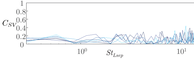
Figure 10: Coherence between PIV v -velocity measurements and unsteady pressure data from the separation duct reference microphone for several points within the separated flow region. The probe locations are denoted by red markers in Figure 8.
