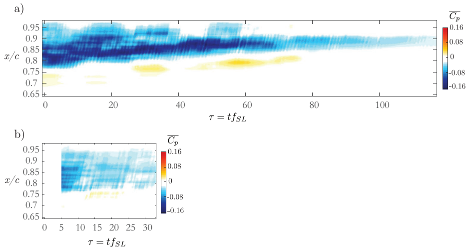
Figure 32: Evolution of moving mean pressure profile at y/c \approx 0.019 for the a) unforced reattachment case and b) adaptive separation control case ( R_{LQR} = 0.5 ). The x-axes for these plots are aligned.
