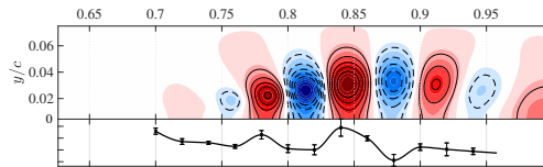
(b) Real part of C_{p'} TDMD mode at St = 1.92 with the online DMD mode from the microphone array shown along the bottom for comparison.
