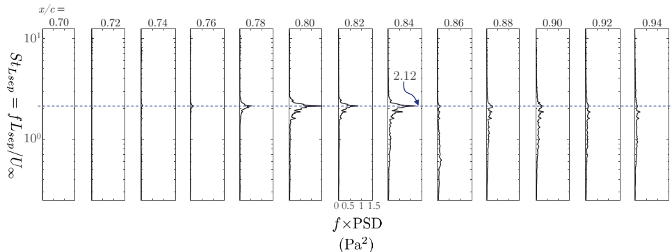
Figure 11: Premultiplied power spectral density plots of the surface mounted microphone array measurements. The microphone location for each plot is denoted at the top of the plot.
