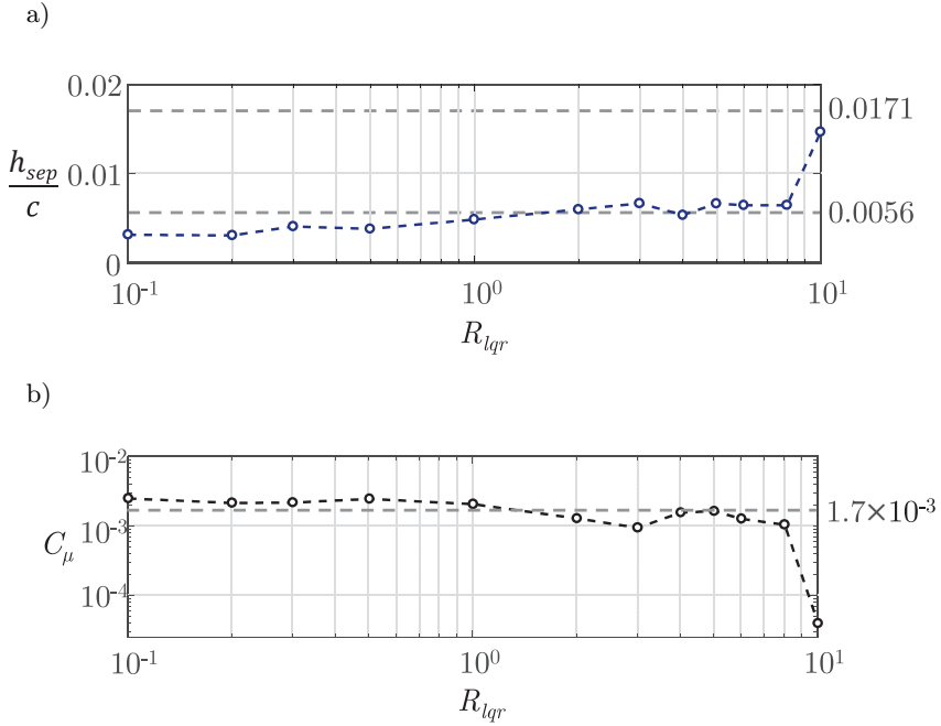
Figure 23: a) Mean separation height and b) actuator input as R_{LQR} is varied. The smallest bubble height occurs for R_{LQR} = 0.2 . For R_{LQR} < 1 , the separation height is h_{sep}/c < 0.006 . The baseline separation height of h_{sep}/c = 0.0171 and the lowest open-loop separation height of h_{sep}/c = 0.0056 are denoted by the dashed gray line. The momentum coefficient corresponding to this open-loop case is also provided ( C_\mu = 1.7 \times 10^{-3} ).
