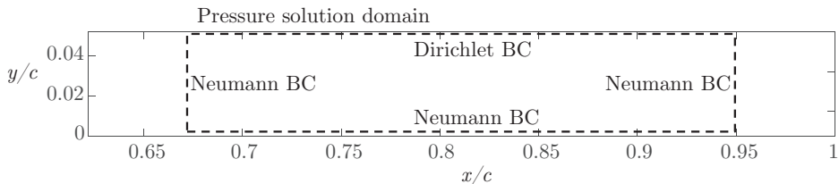
Figure 30: Bounds of the region in which the moving mean pressure field is solved for by the Pressure-Poisson equation.
