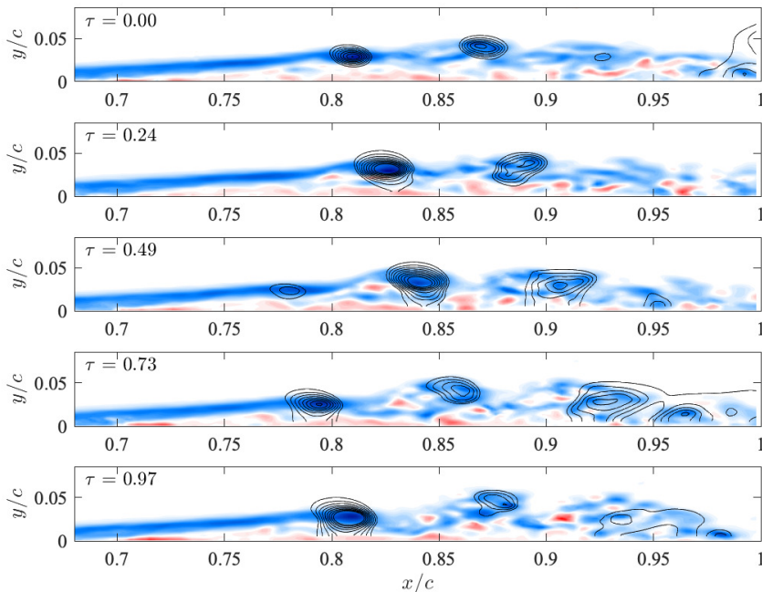
Figure 16: Snapshots of vorticity superimposed with mean-subtracted C_{p'} contours computed from the 2-D PIV vector field. Negative C_{p'} contours are depicted with an increment of 0.05. Regions of low pressure convect with the vortices in the separated shear layer with an average velocity of 0.55U_\infty .
