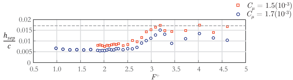
Figure 22: Normalized mean separation height plotted against input frequency. The minimum mean separation height measured corresponds to forcing near the dominant frequency identified by DMD, F^+ \approx 2 . The baseline separation height of h_{sep}/c = 0.0171 is denoted by the dashed gray line.
