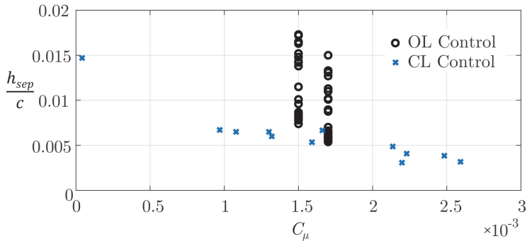
Figure 24: Mean separation bubble height plotted versus momentum coefficient for both open-loop and adaptive closed-loop control.
