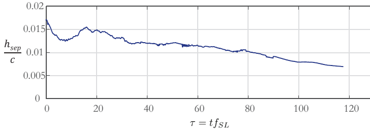
Figure 21: Running calculation of the mean separation height to illustrate the transient response of the flow to turning off the separation system. Each moving mean calculation is comprised of 1250 PIV snapshots (approximately 10 shear layer periods).
