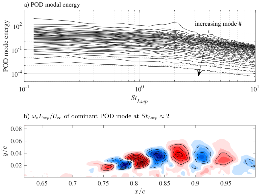
Figure 12: POD of baseline uncontrolled TR-PIV velocity field. (a) POD modal energy vs. Strouhal number and (b) real part of the dimensionless vorticity of the dominant POD mode at St \approx 2 . Dashed contour lines are shown for negative values and solid contour lines for positive values with an increment of 0.03.
