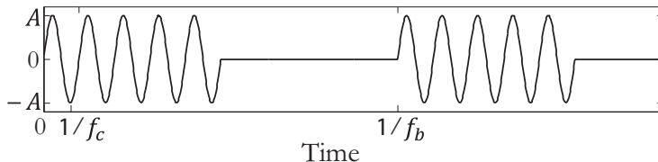
Figure 6: Burst modulation waveform used for periodic actuation corresponding to 50% duty cycle. In this case f_c = 2050 Hz.
