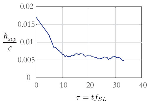
Figure 27: Running calculation of the mean separation height to illustrate the transient response of the flow to adaptive LQR control for R_{lqr} = 0.5 . This is computed from estimating the mean within a time window of \tau = 10 characteristic periods (ensembles of 1250 PIV snapshots).
