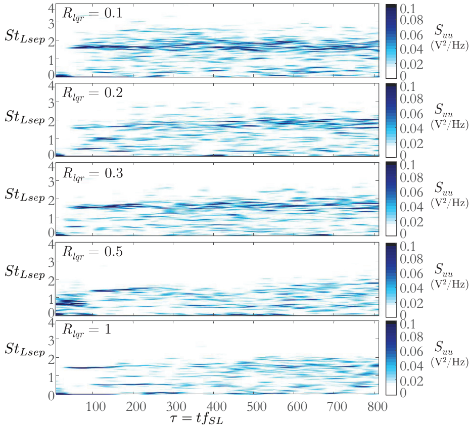
Figure 25: The frequency content of the actuation signal plotted with respect to shear layer periods as a PSD spectrogram. This shows that the input signal exhibits time-varying and broadband frequency content and takes on multiple frequencies simultaneously.
