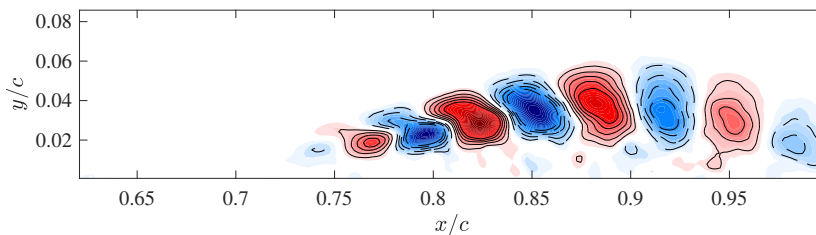
Figure 14: Real part of the dimensionless vorticity for the dominant TDMD mode at St \approx 2 with a reduced rank of r = 25 . Same plot settings as in Figure 12(b).
