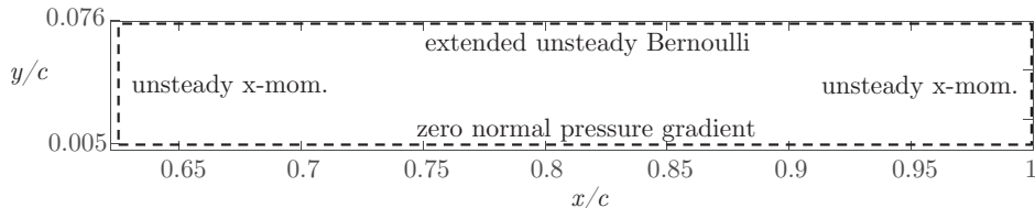
Figure 15: Boundary conditions and domain for solution of the pressure-Poisson equation.
