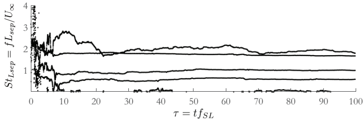
Figure 20: DMD frequencies identified by online DMD with a retention factor of \kappa = 0.99995 .
