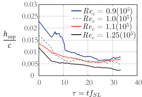
Figure 36: Running calculation of the mean separation height to illustrate the transient response of the flow to adaptive separation control for varying Reynolds numbers. This is computed from the mean of a time window of \tau = 10 characteristic periods (ensembles of 1250 PIV snapshots).
