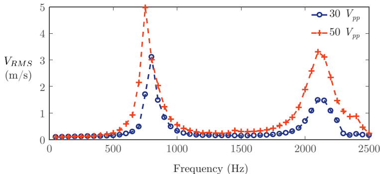
Figure 3: Velocity frequency response for driving amplitudes of 30 and 50 V_{pp} in the slot center above Disk 1.
