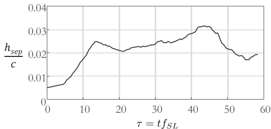
Figure 29: Running calculation of the mean separation height to illustrate the transient response of the flow when adaptive control turned off. The moving mean is estimated over a time window of \tau = 10 characteristic periods (1250 PIV snapshots).
