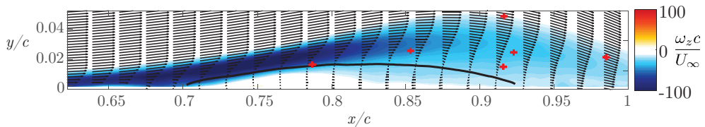
Figure 8: Average z -vorticity as computed from PIV snapshots. The black line denotes the time-averaged \bar{u} = 0 contour. The red markers denote the probe locations from which data are extracted for the coherence estimates in Figure 10.
