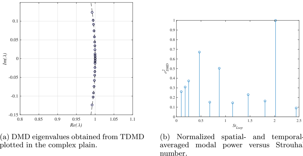
Figure 13: TDMD analysis of baseline uncontrolled TR-PIV velocity field with reduced rank of 25.
