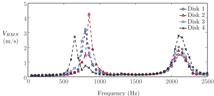
Figure 4: Velocity frequency responses in slot center above all four disks for a driving amplitude of 30 V_{pp} .
