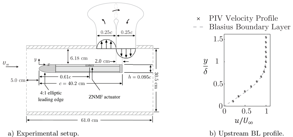
Figure 1: a) Schematic of the flat plate model and flow separation system. The location of the surface microphones are depicted by blue markers. b) Mean velocity profile upstream of the separation point extracted by PIV measurements. The Blasius laminar boundary layer solution is plotted for reference. x/c \approx 0.3 .
