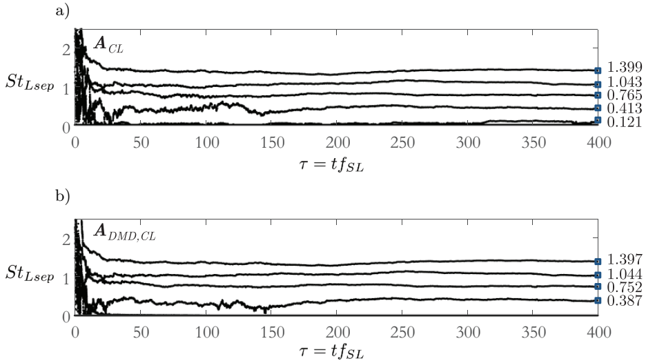
Figure 34: Frequencies of the closed-loop eigenvalues a) determined by online DMD with control by computing \mathbf{A}_{CL} = \mathbf{A}_{DMD} - \mathbf{B}_{DMD}\mathbf{K}_{LQR} and b) by direct estimation of the closed-loop dynamics by online DMD ( \mathbf{A}_{DMD,CL} ). The frequency estimates for \tau = 400 are provided for each plot for comparison.
