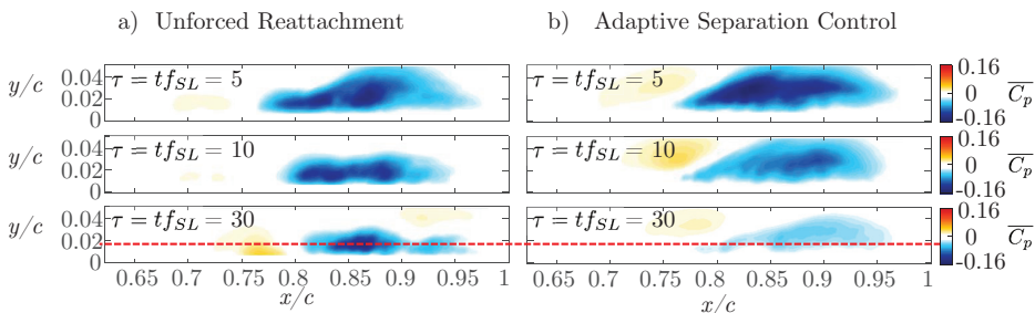
Figure 31: Moving calculation of the mean pressure field. This is computed from moving time window of \tau = 10 characteristic periods (ensembles of 1250 PIV snapshots). The red dashed line depicts the location of the pressure profile extracted for Figure 32.
