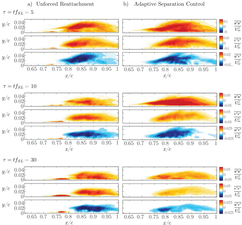
Figure 28: Running calculation of the Reynolds stress components illustrate the evolution of the turbulent stresses subject to unforced reattachment vs. adaptive control ( R_{LQR} = 0.5 ). This is computed over a time window of \tau = 10 characteristic periods (ensembles of 1250 PIV snapshots).
