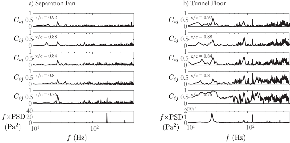
Figure 9: Coherence computed between select surface pressure microphones and the (a) separation fan reference microphone and the (b) tunnel floor reference microphone. The microphone location for each plot is denoted at the top left of the plot. The last graph in each column provides the premultiplied power spectral density for each reference microphone.
