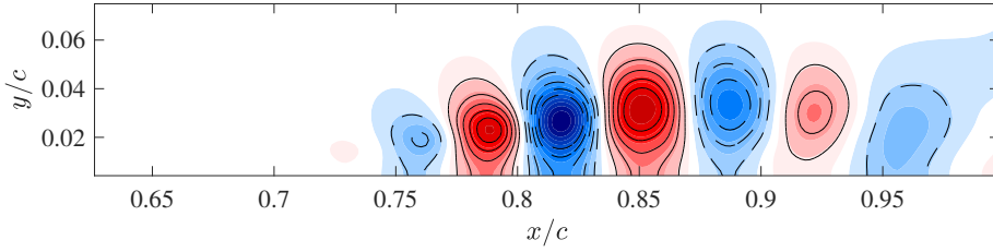
Figure 17: Real part of the dominant POD mode at St \approx 2 applied to n = 10\,000 snapshots of the instantaneous C_{p'} fields using the same settings as in Figure 12(b).
