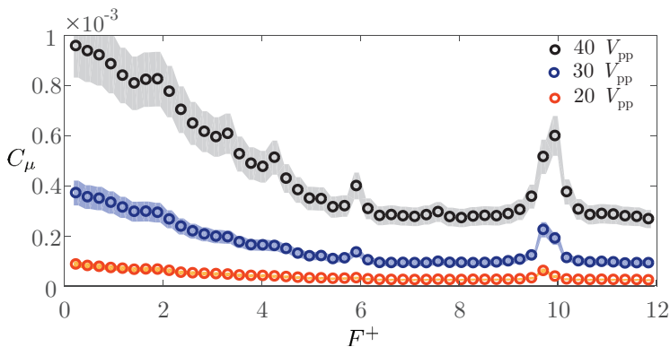
Figure 7: Momentum coefficient with respect to varying forcing frequencies. The 95% confidence intervals are depicted by the shaded region.
