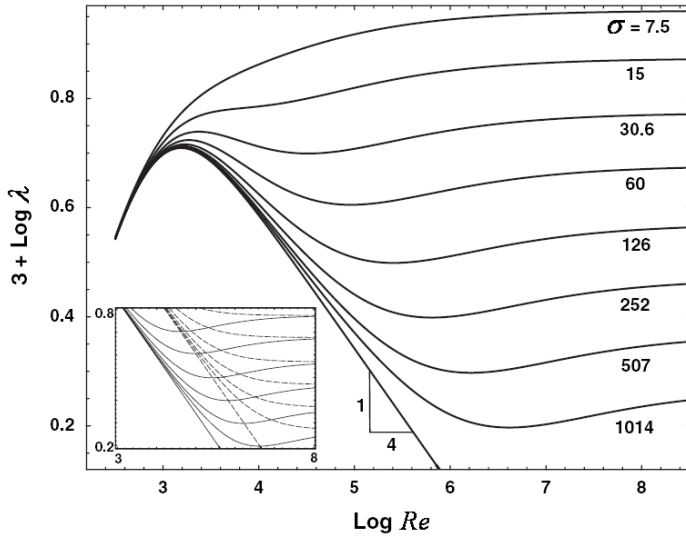
Figure 4: Friction factor curves produced by the analytic model of Gioia and Chakraborty (2006) (cf. figure 5).
