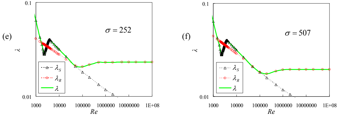
Figure A10: The merge of the final correlations for smooth pipe and rough pipes with six values of roughnesses. \lambda_S and \lambda_R are merged to be \lambda = f(Re, \sigma) for “Virtual Nikuradse”.
