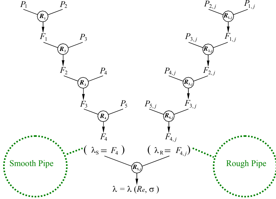
Figure 6: Correlation tree for smooth and rough pipes. P_i and P_{i,j} are power laws, F_i and F_{i,j} are rational fractions of power laws. R_i are branch points for smooth pipe and R_{i,j} are branch points for rough pipes. At each branch point, two assembly member functions are merged into a rational fraction of power laws by processing data with the logistic dose function algorithm. The chain on the left is for smooth pipes and leads to a rational fraction correlation F_4 . The six chains on the right are for rough pipes and lead to six rough pipe correlations F_{4,j} ( j = 1, 2, 3, 4, 5, 6 ). In the correlation tree, \lambda_S = \lambda_S(Re) = F_4(Re) and \lambda_R = \lambda_R(Re, \sigma) = F_{4,j}(Re, \sigma_j) . These correlations are merged into a single composite correlation \lambda = f(Re, \sigma) .
