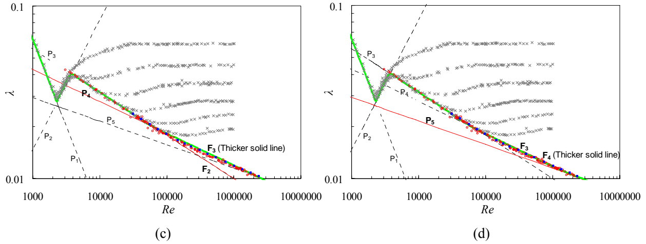
Figure A4: Sequential construction of the correlation tree for smooth pipes. In each of the four panels the straight lines are power laws fit to the data at five places. In panel (a), two power laws P_1 and P_2 are composed into a rational fraction F_1 . In panel (b), P_3 is composed with F_1 to get F_2 . In panel (c), P_4 is composed with F_2 to get F_3 . In panel (d), P_5 is composed with F_3 to get F_4 which gives the final formula giving friction factors vs. Reynolds numbers in smooth pipes (i.e. \lambda_S = F_4 ).
