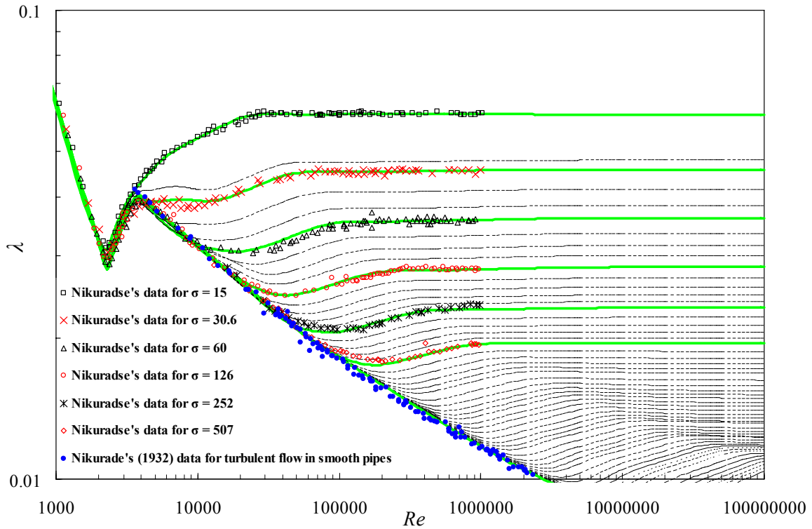
Figure 3: Virtual Nikuradse. Correlations \lambda = f(Re, \sigma) for values of \sigma are up to 10^5 , computed from equation (5). Nikuradse's (1933) data for rough pipes and (1932) data for smooth pipe are included for comparison. The solid green lines are the data fits shown in figure 2. The dotted curves between and beyond the data fits are virtual curves obtained from equation (5) predicting the results of experiments not yet done.
