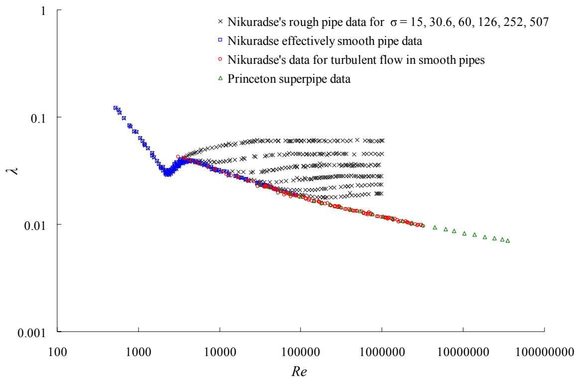
Figure 1: Friction factor vs. Reynolds number. The data from Nikuradse (1932) for flow in smooth pipes, the data from Nikuradse (1933) for effectively smooth turbulent flow in rough pipes and data from the Princeton superpipe coincide. Data in the transition region is influenced strongly by instabilities that depend on many parameters and is better described as data cloud rather than a data curve.
