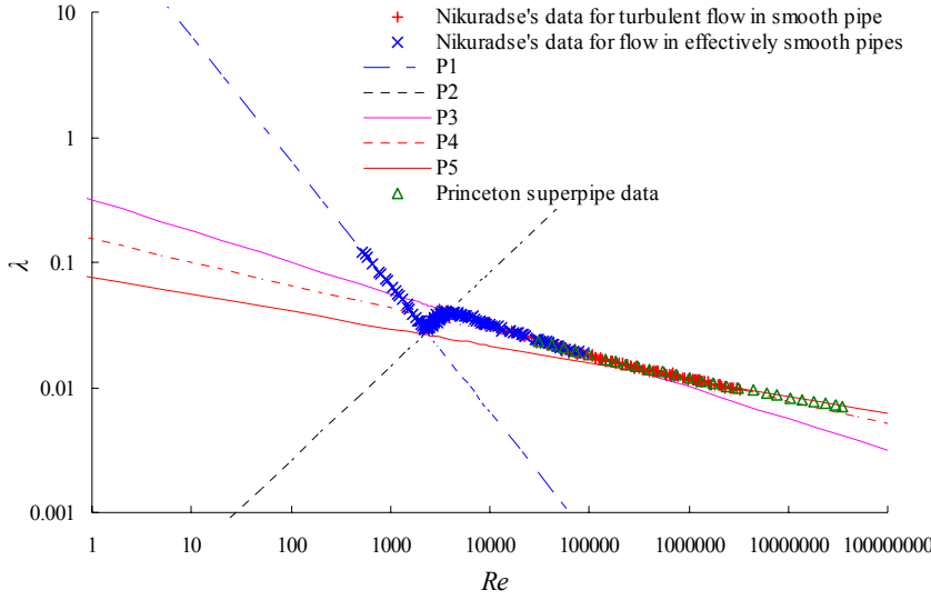
Figure A2: Nikuradse's (1932) and Princeton data for flow in smooth and effectively smooth pipes. Five branches of power laws are identified in the graph. They are P_i ( i = 1, 2, 3, 4, 5 ) in equation (A.2).
