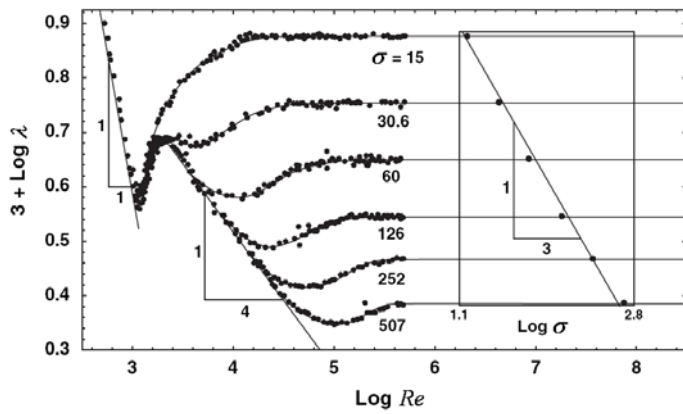
Figure 5: [After Goia & Chakraborty (2006)] Nikuradse's (1933) data for the friction factor vs. Reynolds number emphasizing the Blasius 1/4 law and Strickler's \sigma^{-1/3} correlation at large Reynolds numbers. Our processing of the Nikuradse's data does not lead to Strickler's correlation (see equation (5)) and it does not lead to the Blasius law (see equation (4)).
