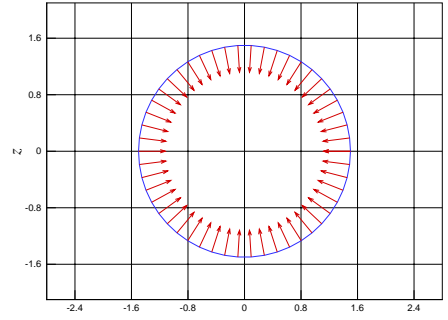
(d) (T_{nn}n_y + T_{nn}n_z) dyn/cm 2 for an ellipsoid y^2/b^2 + z^2/c^2 = 1 - x^2/a^2 with x = 0.0 cm, in the (y, z) -plane.
