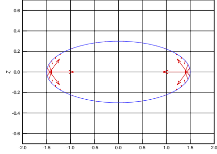
(d) (T_{nn}n_y + T_{nn}n_z)/10 dyn/cm 2 for an ellipsoid y^2/b^2 + z^2/c^2 = 1 - x^2/a^2 with x = 0.0 cm, in the (y, z) -plane.
