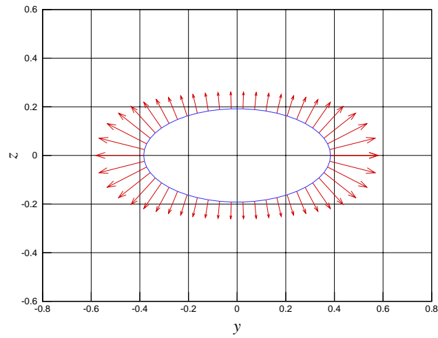
Figure 13: Normal stress (T_{nn}n_y + T_{nn}n_z) / 600 \text{ dyn/cm}^2 for an ellipse y^2/b^2 + z^2/c^2 = 1 - 2.9^2/a^2 at x = 2.9 \text{ cm} in the (y, z) -plane. Perpendicular view of the cross section (i) in figure 4. The strong tension observed near the trailing stagnation point may explain the formation of a two-dimensional cusping tail in a gas bubble rising in viscoelastic fluids.
