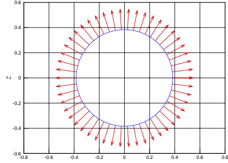
(f) (T_{nn}n_y + T_{nn}n_z)/250 dyn/cm 2 for an ellipsoid y^2/b^2 + z^2/c^2 = 1 - x^2/a^2 with x = 2.9 cm, in the (y, z) -plane.
