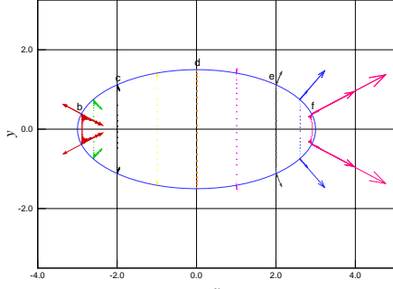
(a) (T_{nn}n_x + T_{nn}n_y)/1200 dyn/cm 2 for an ellipsoid x^2/a^2 + y^2/b^2 = 1 - z^2/c^2 with z = 0 , in the (x, y) -plane.
