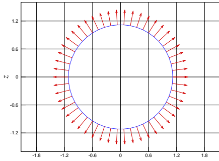
(e) (T_{nn}n_y + T_{nn}n_z)/50 dyn/cm 2 for an ellipsoid y^2/b^2 + z^2/c^2 = 1 - x^2/a^2 with x = 2.0 cm, in the (y, z) -plane.
