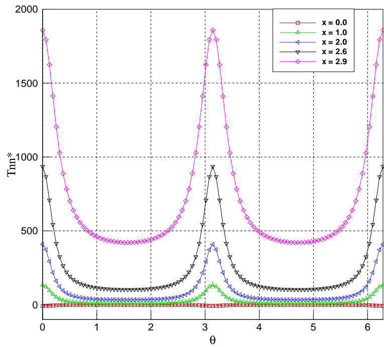
Figure 15: Dimensionless normal stress as a function of the polar angle \theta for the different cross sections of the rear part of the ellipsoid shown in figures 9 to 13 ( x \geq 0 ). The normal stress is tension in the rear of the ellipsoid, with a strong tension near the trailing edge.
