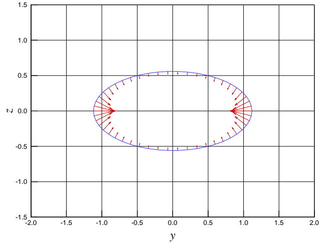
Figure 7: Normal stress (T_{nn}n_y + T_{nn}n_z) / 150 \text{ dyn/cm}^2 for an ellipse y^2/b^2 + z^2/c^2 = 1 - 2.0^2/a^2 at x = -2.0 \text{ cm} in the (y, z) -plane. Perpendicular view of the cross section (c) in figure 4. Strong compression at the right and left poles of the ellipse and mild compression towards the center.
