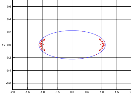
(c) (T_{nn}n_y + T_{nn}n_z)/800 dyn/cm 2 for an ellipsoid y^2/b^2 + z^2/c^2 = 1 - x^2/a^2 with x = -2.0 cm, in the (y, z) -plane.
