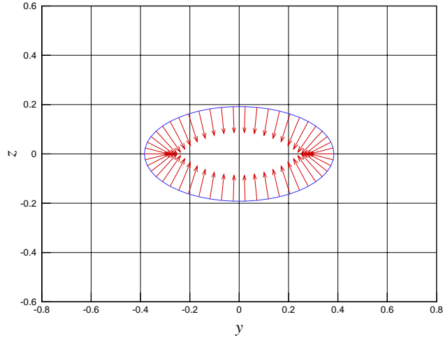
Figure 5: Normal stress (T_{nn}n_y + T_{nn}n_z)/600 \text{ dyn/cm}^2 for an ellipse y^2/b^2 + z^2/c^2 = 1 - 2.9^2/a^2 at x = -2.9 \text{ cm} in the (y, z) -plane. Perpendicular view of the cross section (a) in figure 4. The normal stress at the front of the ellipsoid gives rise to compression near the leading edge. This may explain the flat top observed in gas bubbles rising in viscoelastic fluids (see figure 1).
