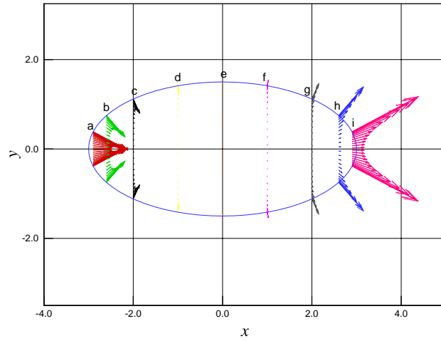
Figure 4: Distribution of the normal stress at the surface of a tri-axial ellipsoid, immersed in a uniform stream that moves from left to right. Two-dimensional representation in the (x, y) -plane of an ellipsoid (with semi-axes a = 3 , b = 1.5 , c = 0.75 cm). The arrows represent the normal stress (T_{nn}n_x + T_{nn}n_y) / 150 dyn/cm 2 evaluated for different cross sections along the ellipsoid. The cross sections are located at: x = -2.9 (a), -2.6 (b), -2.0 (c), -1.0 (d), 0.0 (e), 1.0 (f), 2.0 (g), 2.6 (h) and 2.9 (i) cm. A perpendicular view of the different cross sections is shown in figures 5-13. There is compression in the fore part of the ellipsoid and a strong tension in the rear, near the trailing stagnation point.
