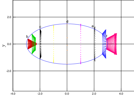
(a) (T_{nn}n_x + T_{nn}n_y)/100 dyn/cm 2 for an ellipsoid x^2/a^2 + y^2/b^2 = 1 - z^2/c^2 with z = 0 , in the (x, y) -plane.
