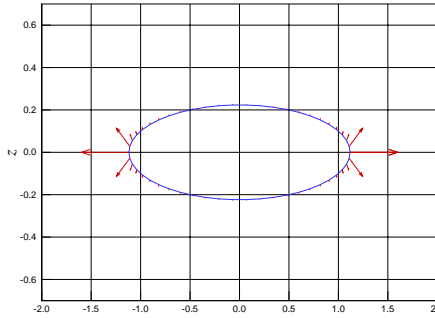
(e) (T_{nn}n_y + T_{nn}n_z)/800 dyn/cm 2 for an ellipsoid y^2/b^2 + z^2/c^2 = 1 - x^2/a^2 with x = 2.0 cm, in the (y, z) -plane.
