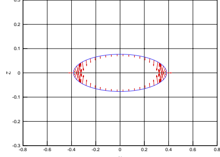
(b) (T_{nn}n_y + T_{nn}n_z)/7500 dyn/cm 2 for an ellipsoid y^2/b^2 + z^2/c^2 = 1 - x^2/a^2 with x = -2.9 cm, in the (y, z) -plane.
