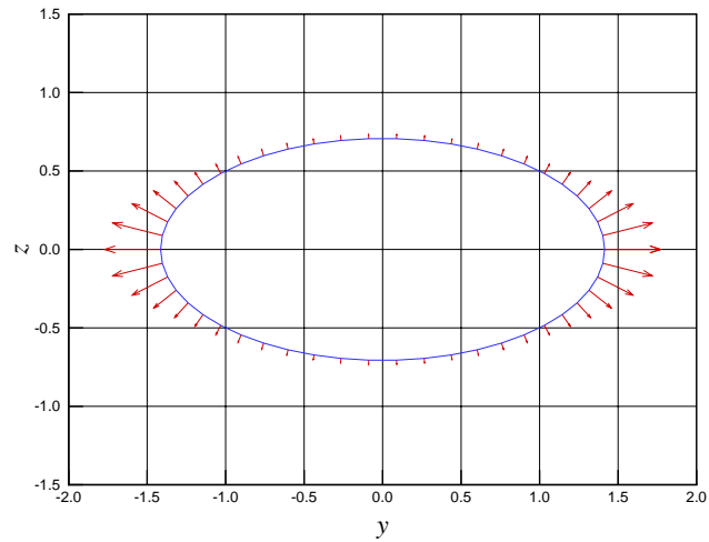
Figure 10: Normal stress (T_{nn}n_y + T_{nn}n_z) / 50 \text{ dyn/cm}^2 for an ellipse y^2/b^2 + z^2/c^2 = 1 - 1.0^2/a^2 at x = 1.0 \text{ cm} in the (y, z) -plane. Perpendicular view of the cross section (f) in figure 4. There is a change of sign of the normal stress right after the front half of the ellipsoid. It changes from negative (compression) to positive (tension). Strong tension near the right and left poles and mild tension towards the center. This may induce the formation of a flat tail for a gas bubble. The same effect is observed in the other cross sections of the rear part of the ellipsoid (see figures 11-13) .
