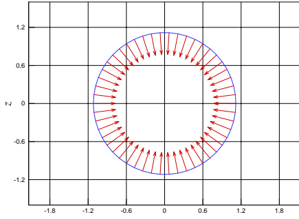
(c) (T_{nn}n_y + T_{nn}n_z)/50 dyn/cm 2 for an ellipsoid y^2/b^2 + z^2/c^2 = 1 - x^2/a^2 with x = -2.0 cm, in the (y, z) -plane.
