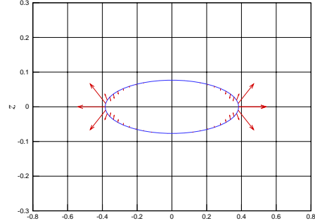
(f) (T_{nn}n_y + T_{nn}n_z)/7500 dyn/cm 2 for an ellipsoid y^2/b^2 + z^2/c^2 = 1 - x^2/a^2 with x = 2.9 cm, in the (y, z) -plane.
