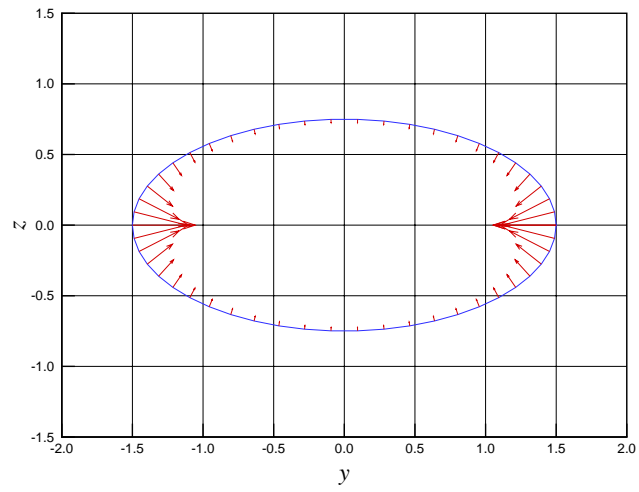
Figure 9: Normal stress (T_{nn}n_y + T_{nn}n_z)/2.5 \text{ dyn/cm}^2 for an ellipse y^2/b^2 + z^2/c^2 = 1 at x = 0.0 \text{ cm} in the (y, z) -plane. Perpendicular view of the cross section (e) in figure 4. There is still compression right in the middle of the ellipsoid.
