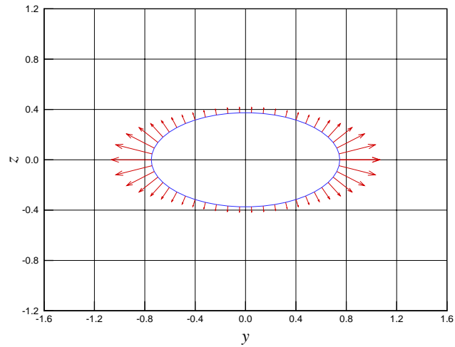
Figure 12: Normal stress (T_{nn}n_y + T_{nn}n_z)/300 \text{ dyn/cm}^2 for an ellipse y^2/b^2 + z^2/c^2 = 1 - 2.6^2/a^2 at x = 2.6 \text{ cm} in the (y, z) -plane. Perpendicular view of the cross section (h) in figure 4. Strong tension at the right and left poles, causes the ellipsoid to get flatter.
