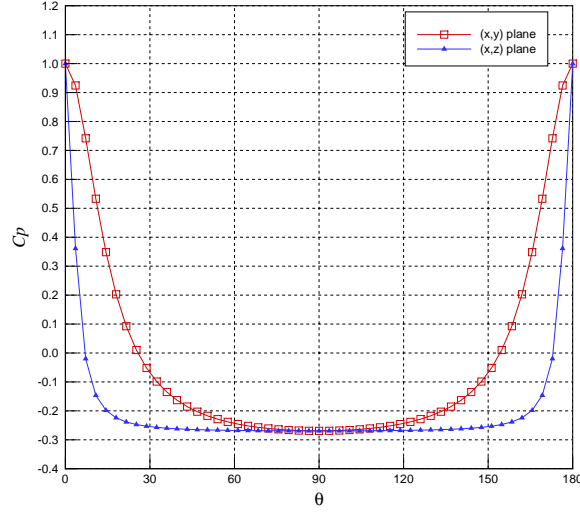
Figure 3: Pressure coefficient distribution on the surface of an ellipsoid for two cross sections in the (x-y) and (x-z) planes with z = 0 and y = 0 respectively.
