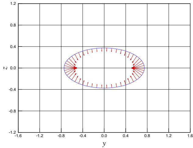
Figure 6: Normal stress (T_{nn}n_y + T_{nn}n_z)/300 \text{ dyn/cm}^2 for an ellipse y^2/b^2 + z^2/c^2 = 1 - 2.6^2/a^2 at x = -2.6 \text{ cm} in the (y, z) -plane. Perpendicular view of the cross section (b) in figure 4. There is a bigger compression (indicated by bigger inwards arrows) at the right and left poles of the ellipse. This may cause that the cross section of the ellipsoid becomes more round and in consequence the ellipsoid would tend to be prolate.
