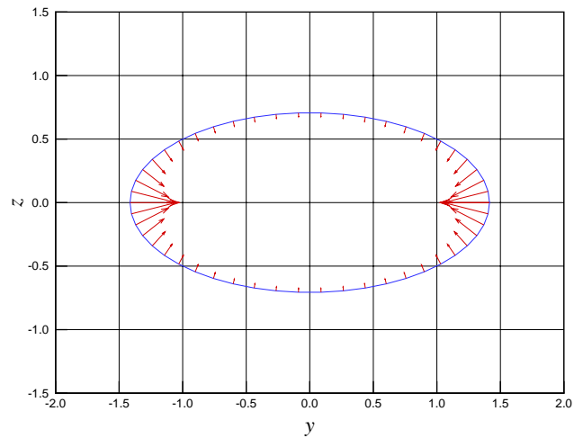
Figure 8: Normal stress (T_{nn}n_y + T_{nn}n_z) / 50 \text{ dyn/cm}^2 for an ellipse y^2/b^2 + z^2/c^2 = 1 - 1.0^2/a^2 at x = -1.0 \text{ cm} in the (y, z) -plane. Perpendicular view of the cross section (d) in figure 4. Small compression at the center and high compression at the right and left poles of the ellipse (indicated by small and big inwards arrows). This suggests that the upper part of a gas bubble rising in a viscoelastic fluid would tend to be prolate.
