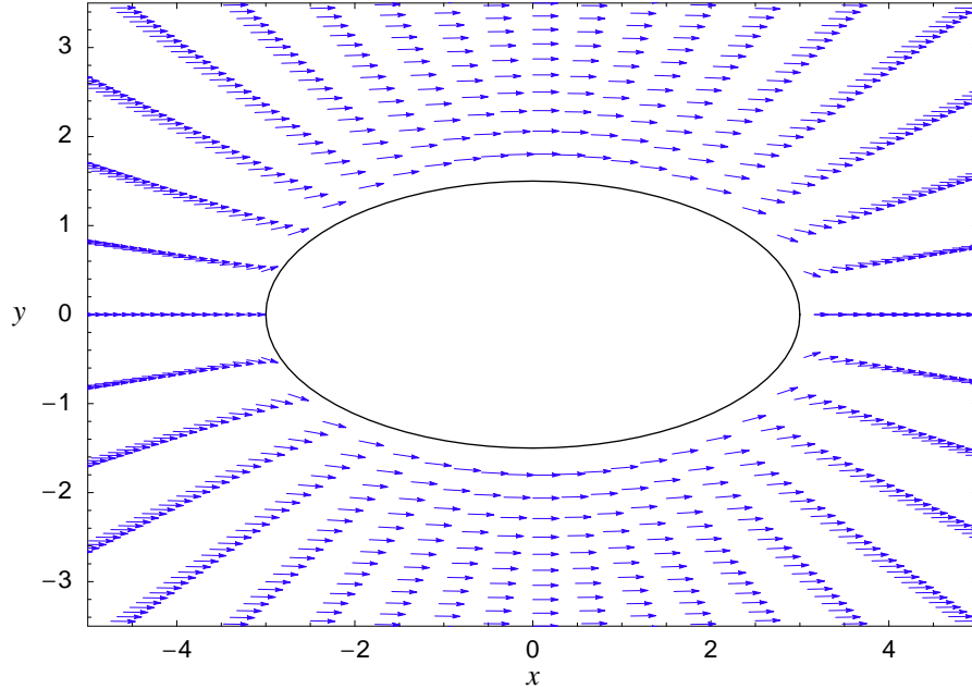
Figure 2: Velocity field of an irrotational, inviscid flow around an ellipsoid with semi-axes a = 3 , b = 1.5 , c = 0.75 , and a Reynolds number of 0.05. Two dimensional representation of the velocity field at the centerline of the ellipsoid ( z = 0 ).
