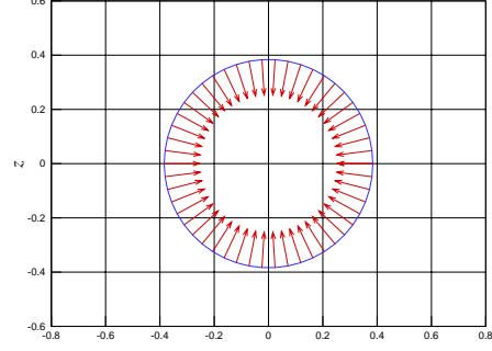
(b) (T_{nn}n_y + T_{nn}n_z)/250 dyn/cm 2 for an ellipsoid y^2/b^2 + z^2/c^2 = 1 - x^2/a^2 with x = -2.9 cm, in the (y, z) -plane.
