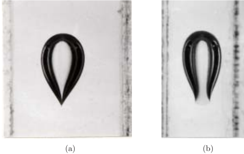
Figure 1: Two orthogonal views showing the cusped (a) and broad (b) shape of the trailing edge of an air bubble ( 2 \text{ cm}^3 ), rising in a viscoelastic liquid (S1). The two photographs are from Liu, Liao & Joseph (1995).
