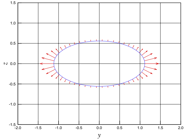
Figure 11: Normal stress (T_{nn}n_y + T_{nn}n_z)/150 \text{ dyn/cm}^2 for an ellipse y^2/b^2 + z^2/c^2 = 1 - 2.0^2/a^2 at x = 2.0 \text{ cm} in the (y, z) -plane. Perpendicular view of the cross section (g) in figure 4. Strong tension at the right and left poles, causes the ellipsoid to get flatter.
