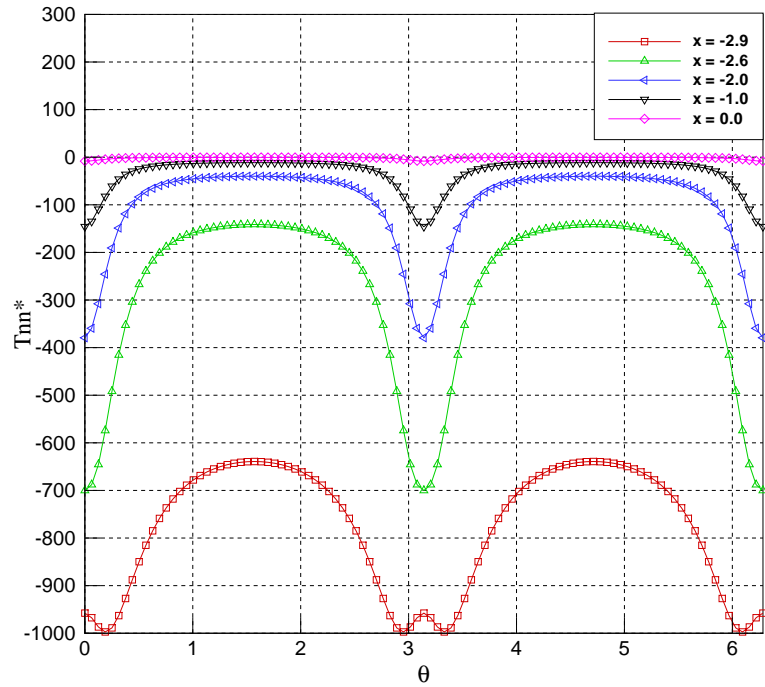
Figure 14: Dimensionless normal stress as a function of the polar angle \theta for the different cross sections of the frontal part of the ellipsoid shown in figures 5 to 9 ( x \leq 0 ). The normal stress is compression in the fore part of the ellipsoid. The maximum compression is observed near the leading edge, and decreases as we move towards the rear of the ellipsoid.
