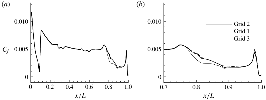
FIGURE 6. Grid convergence for C_f on the hull. Grids 1–3 only differ in the streamwise resolution on the stern ( x/L > 0.56 ), with grid 1 being the coarsest and grid 3 being the finest. The results from grid 2 are presented in this work.
