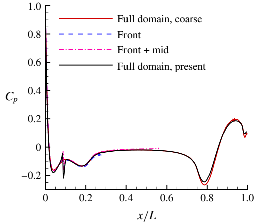
FIGURE 5. (Colour online) Grid convergence for C_p . Results from all the preliminary simulations are compared to the final grid. Note that grids 1–3 give identical C_p , hence only the grid 2 result is shown as the present result.
