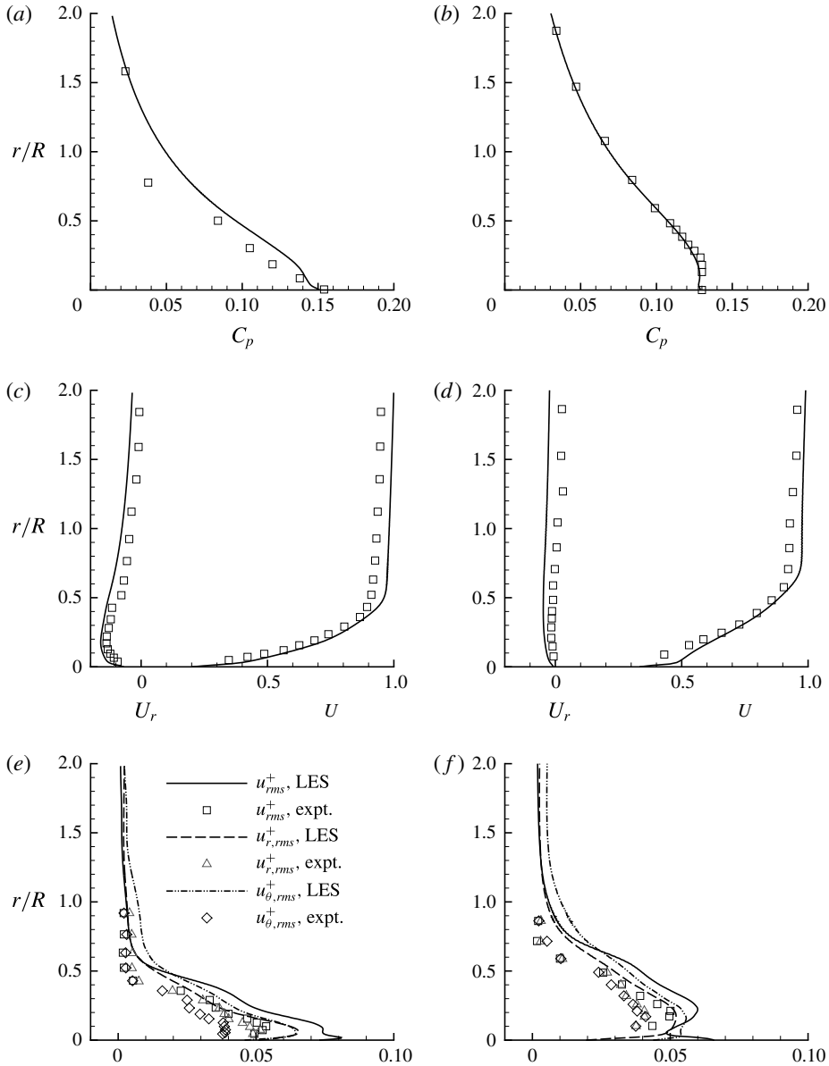
FIGURE 15. Profiles of pressure coefficient ( C_p ) (a,b), mean axial ( U ) and radial ( U_r ) velocity (c,d) and r.m.s. of velocity fluctuations ( u_{rms}^+ , u_{r,rms}^+ and u_{\theta,rms}^+ ) (e,f), at x/L=0.904 (a,c,e) and 0.978 (b,d,f). Symbols show measurements from the experiments of Huang et al. (1992) at Re = 1.2 \times 10^7 .
