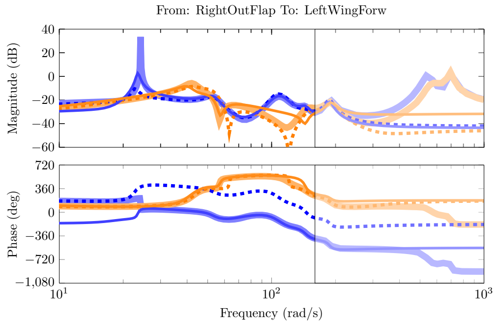
Figure 4.16: Bode plots of full order model (148 states) at 42 KEAS ( — ) and 72 KEAS ( — ) compared to LPV balanced reduced model with 21 states ( - - - / - - - ) and LTI balanced reduced model with 17 states ( — / — ). Lighter areas denote frequency range of no interest.
