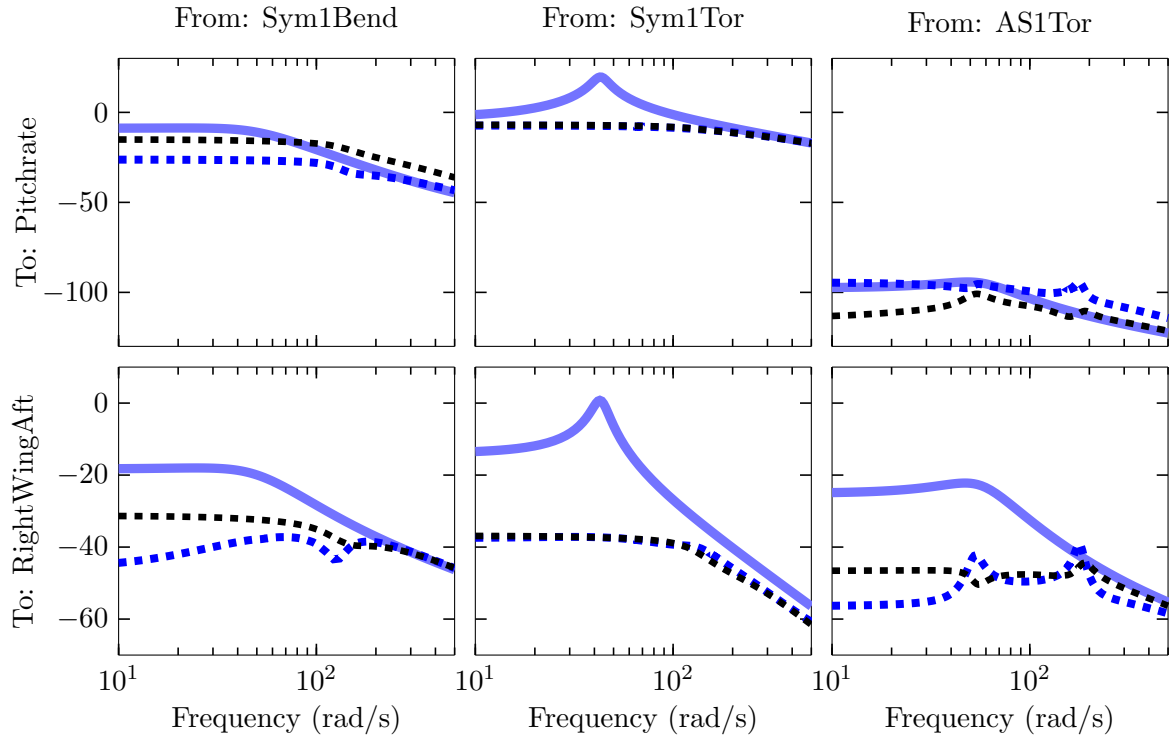
Figure 5.10: Frequency response from the three modal velocity disturbances to the pitch rate and accelerometer in the wing trailing edge for the open-loop system (—), closed-loop system with all sensors available (---), and only accelerometers (---) at 72 KEAS
