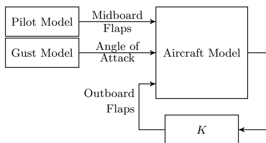
(a) Deflection and rate limit verification model.
