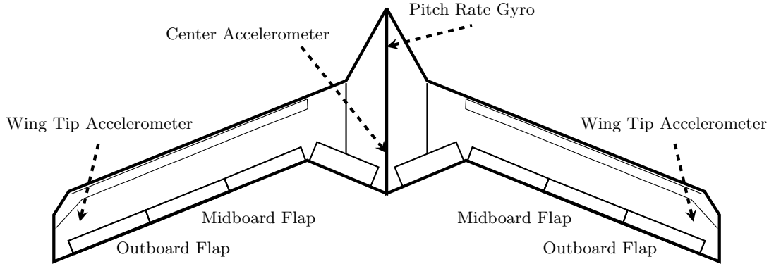
Figure 2. Schematic of the mini MUTT aircraft.
