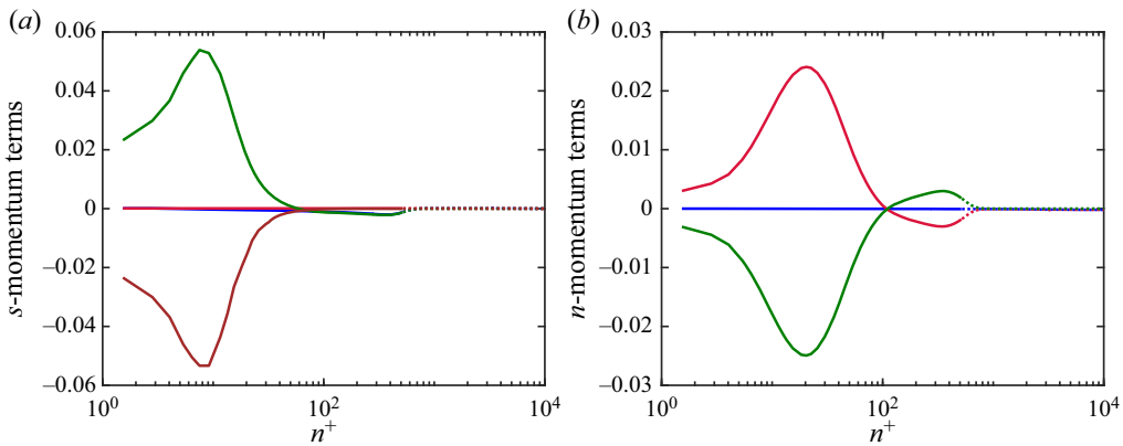
Figure 16. Profiles of terms in the boundary layer equations for the streamline-normal line emanating from x/D = 4.2 on the hull surface (the fourth line from figure 15a). (a) Terms in the streamwise momentum equation: U_s(\partial U_s/\partial s) (blue), -(1/\rho)(\partial P/\partial s) (red), -(1/r)(\partial/\partial n)(r\bar{u}_s\bar{u}_n) (green) and (1/r)(\partial/\partial n)(rv(\partial U_s/\partial n)) (brown). (b) Terms in the streamwise-normal momentum equation: U_s^2/R_s (blue), -(1/\rho)(\partial P/\partial n) (red) and -(1/r)(\partial/\partial n)(r\bar{u}_n^2) (green). All terms are non-dimensionalized using inner scales ( v/u_\tau^2 ). Dotted lines represent points outside of the boundary layer.
