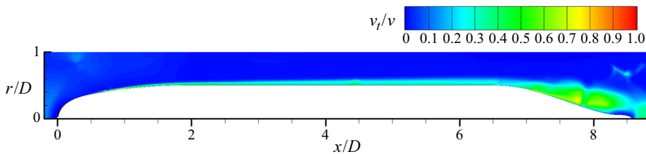
Figure 5. Circumferentially averaged mean eddy viscosity normalized by the molecular viscosity around the hull.
