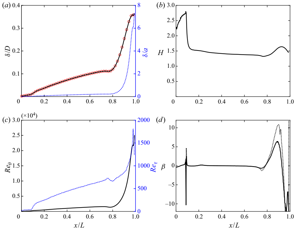
Figure 9. Variation of (a) boundary layer thickness, (b) shape factor, (c) Re_\theta and Re_\tau , and (d) the boundary layer edge (—) and wall (· · · · ·) Clauser pressure gradient parameters versus x/L along the hull. Profiles are extracted along the streamline-normal coordinate direction from lines originating at the hull surface. The red symbols in panel (a) represent \delta/D at intervals along the hull computed using the inviscid velocity method of Griffin et al. (2021).
