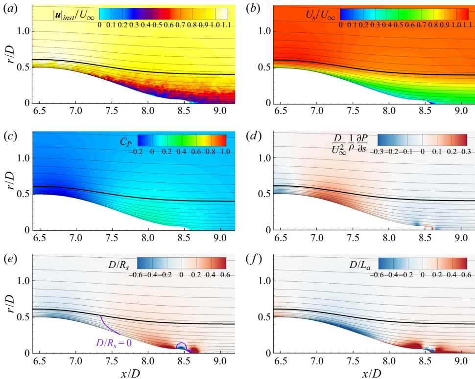
Figure 17. Contours of (a) instantaneous velocity magnitude, (b) U_s/U_\infty , (c) C_p , (d) non-dimensionalized streamwise pressure gradient, (e) D/R_s and (f) D/L_a along with streamlines. The bold line represents the edge of the boundary layer. The purple line in panel (e) marks the streamline curvature inflection line ( D/R_s = 0 ) inside the boundary layer.
